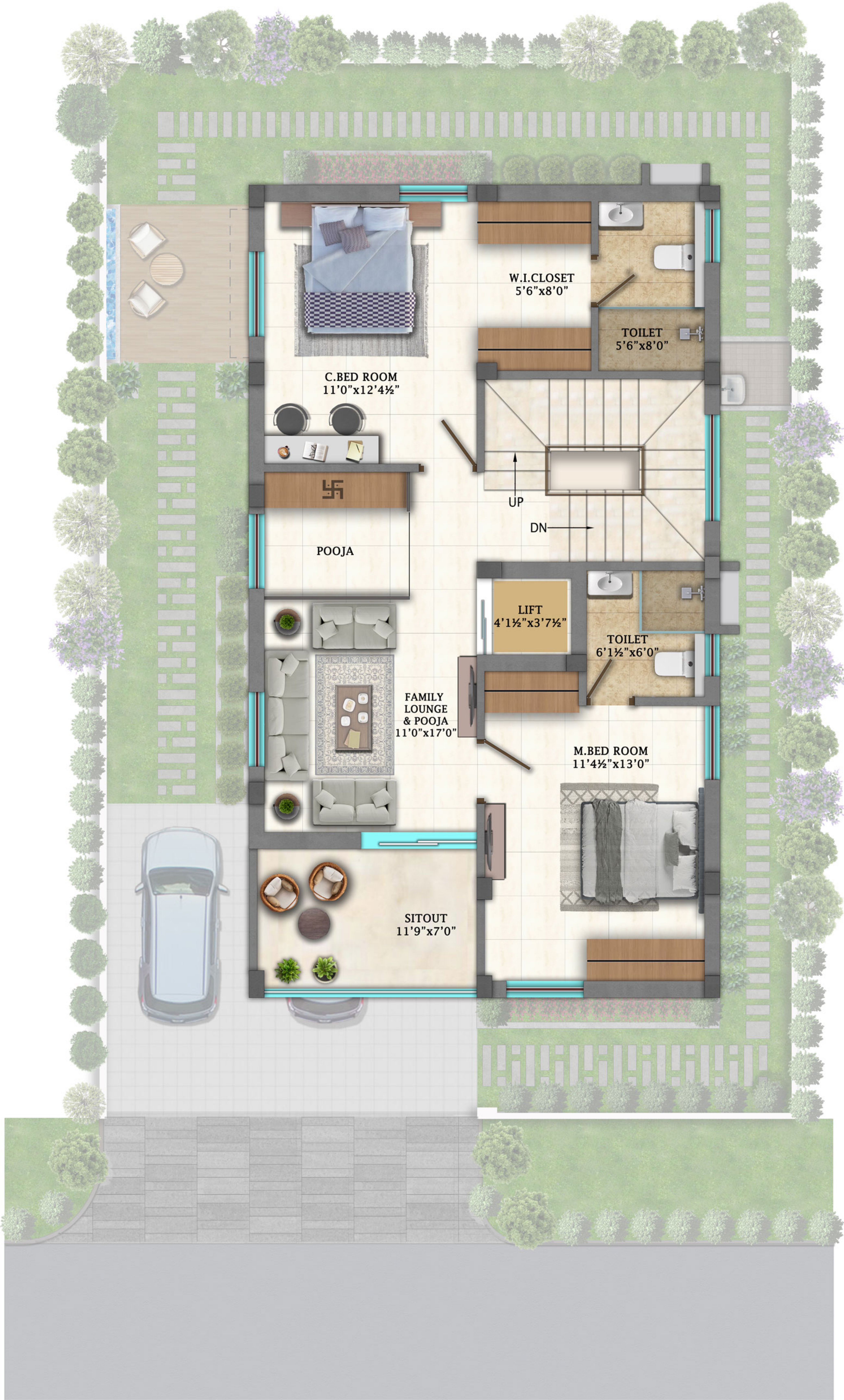
WEST - FIRST FLOOR PLAN
